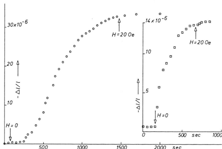
← Fig. 2. Reactivation of the mechanical after-effect of the sample Fe E II due to the kind of experimental conditions described under point 1. of the text. The right-hand curve corresponds to a constant applied pressure of 21.2 kp/mm 2 , the left one was measured under constant pressure of 28 kp/mm 2 .
